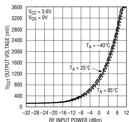
Typical Detector Characteristics, 7GHz
