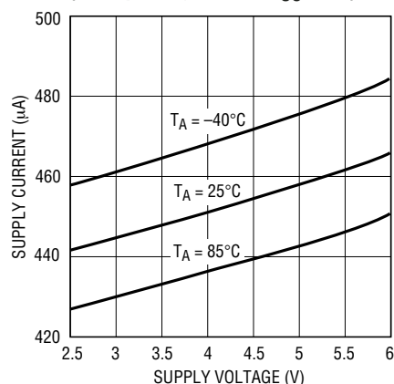
Supply Current vs Supply Voltage (RF Input Signal Off, V_{OS} = 0V )
