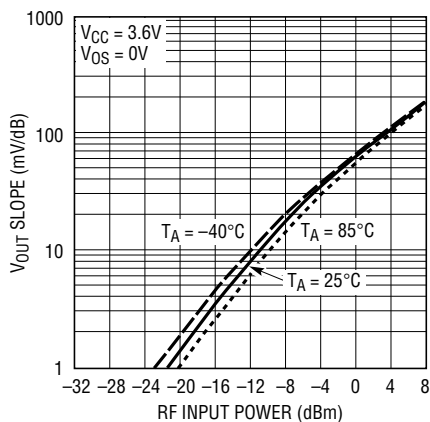
Figure 2. V_{OUT} Slope vs RF Input Power at 11GHz
