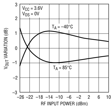
V_{OUT} Variation Relative to 25°C vs RF Input Power at 7GHz
