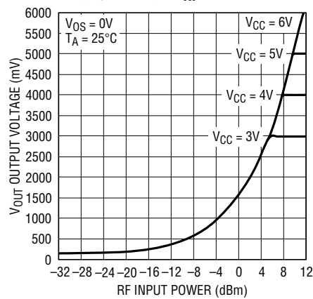
V_{OUT} vs RF Input Power and V_{CC} Supply Voltage, f_{RF} = 2\text{GHz}
