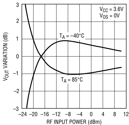
Figure 3. V_{OUT} Variation at -40^{\circ}\text{C} and at 85^{\circ}\text{C} vs RF Input Power at 11GHz, Normalized to Room Temperature ( 25^{\circ}\text{C} ) Results.
