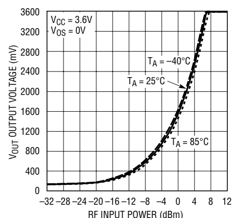
Typical Detector Characteristics, 2GHz
