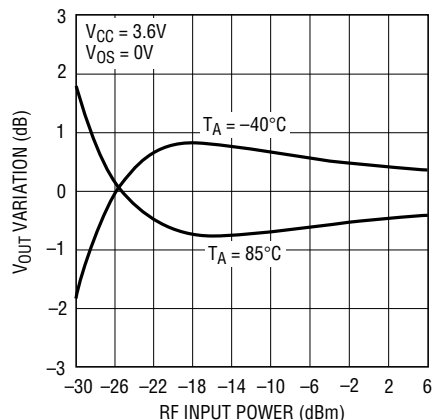
V_{OUT} Variation Relative to 25°C vs RF Input Power at 3GHz
