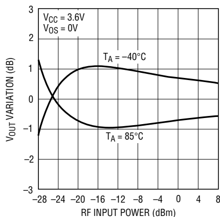
V_{OUT} Variation Relative to 25°C vs RF Input Power at 5GHz
