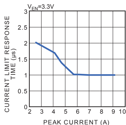
Short Circuit Response Time vs. Peak Current
