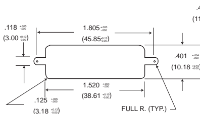
Figure 2 Rear Mounting
