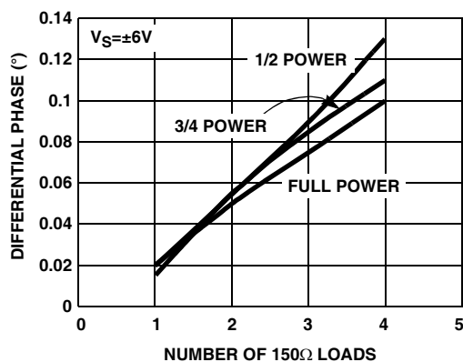
FIGURE 38. DIFFERENTIAL PHASE
