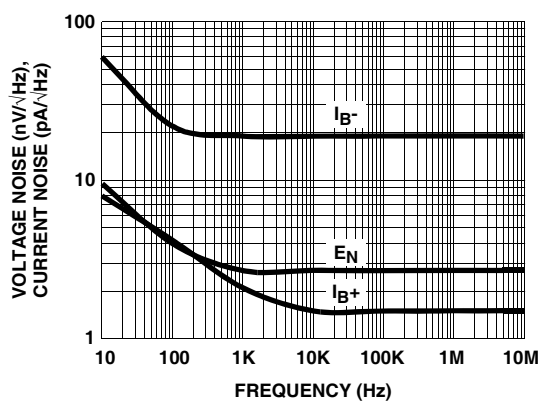
FIGURE 36. VOLTAGE AND CURRENT NOISE vs FREQUENCY
