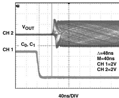
FIGURE 40. ENABLE RESPONSE
