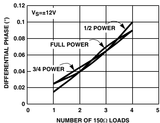
FIGURE 39. DIFFERENTIAL PHASE
