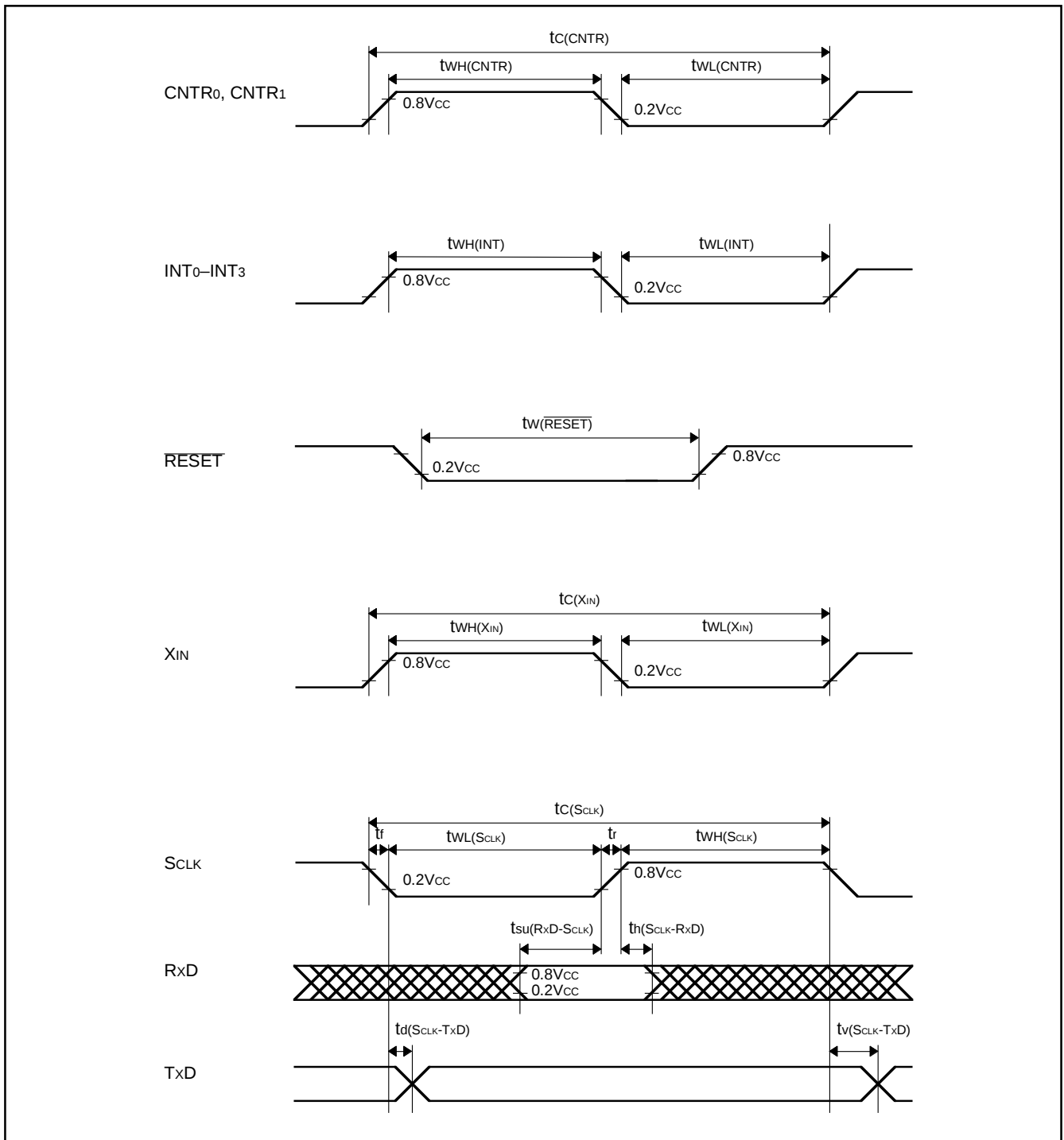
Fig. 53 Timing diagram
