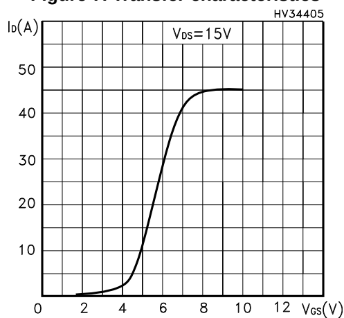
Figure 7. Transfer characteristics
