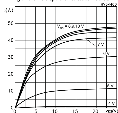
Figure 6. Output characteristics
