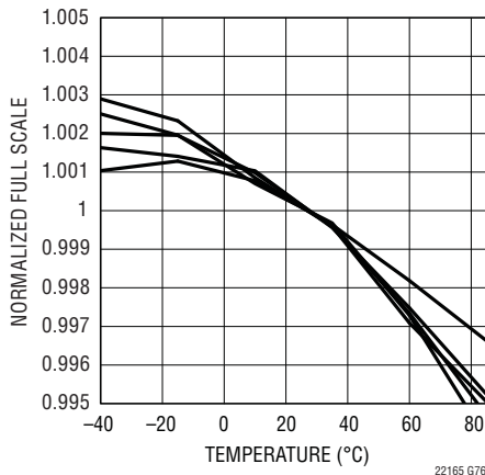
LTC2216/LTC2215 Normalized Full-Scale vs Temperature, Internal Reference, 5 Units
