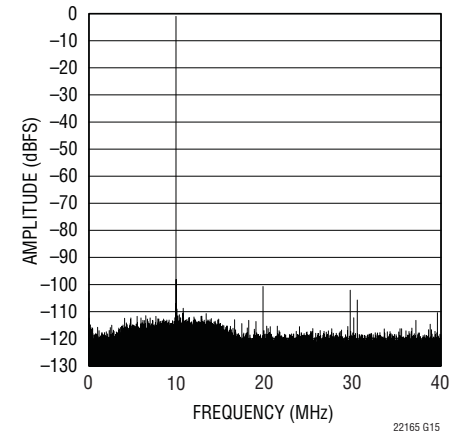
LTC2216 64k Point FFT, f_{IN} = 70.2\text{MHz} , -1\text{dBFS}
