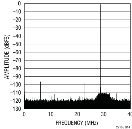
LTC2216 64k Point FFT, f_{IN} = 28.7\text{MHz} , -1\text{dBFS}
