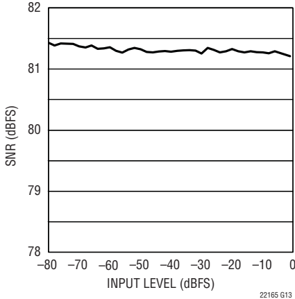
LTC2216 SNR vs Input Level, f_{IN} = 15.2\text{MHz}
