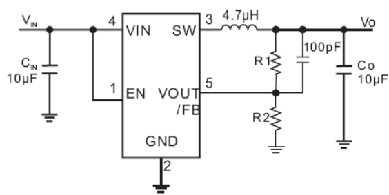
Adjustable Output Voltage
