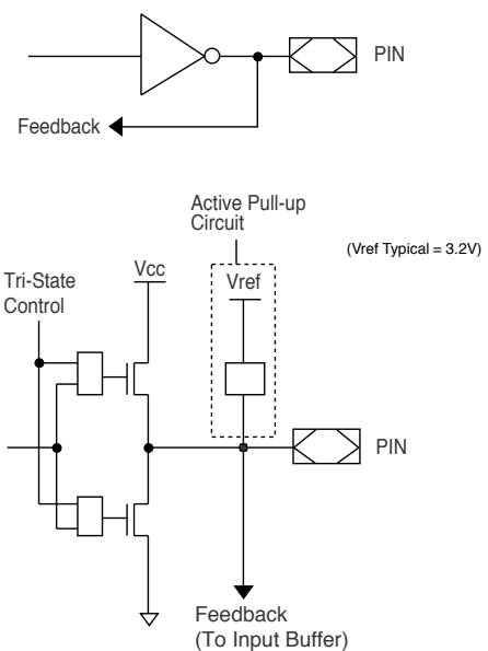
Typical Output
