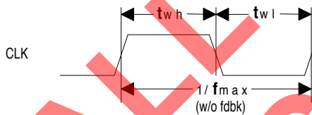
Clock Width
