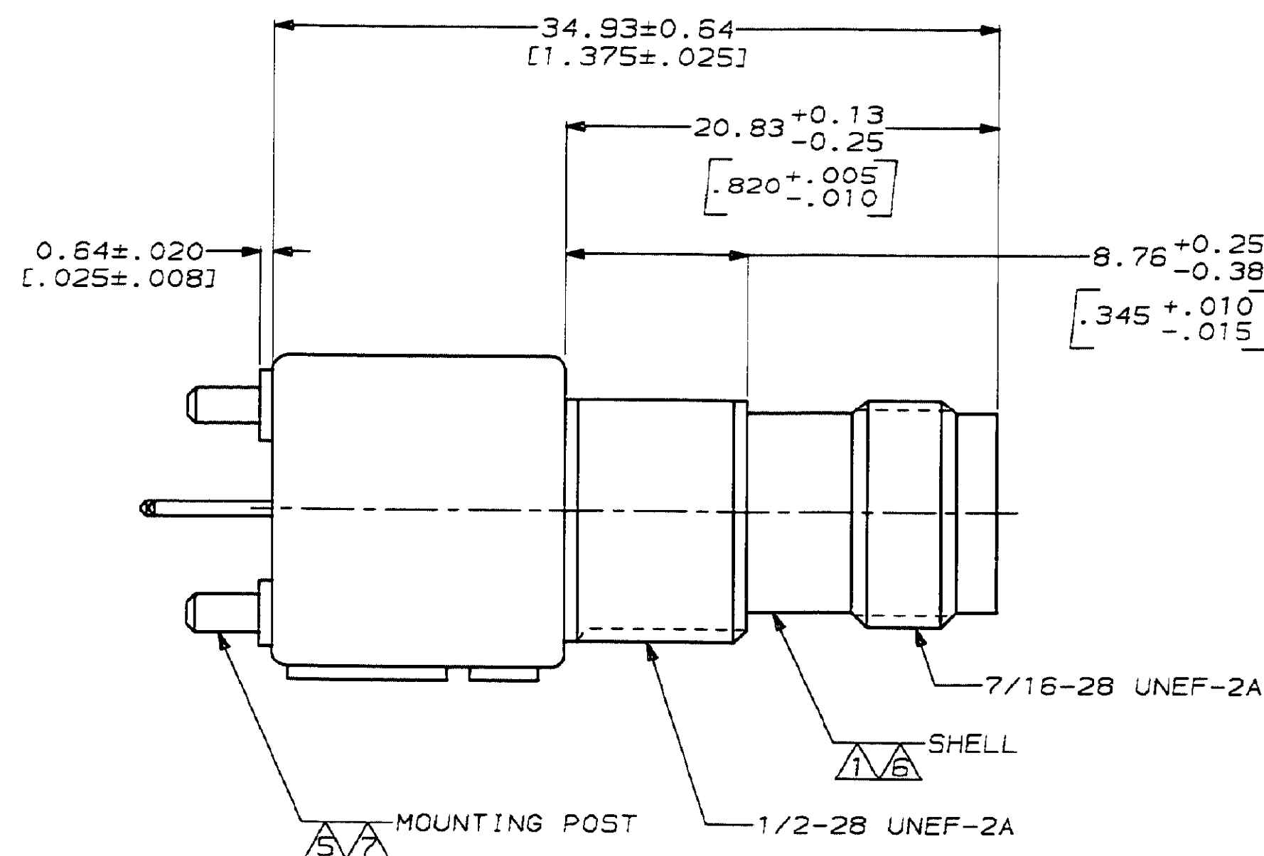
VIEW A
