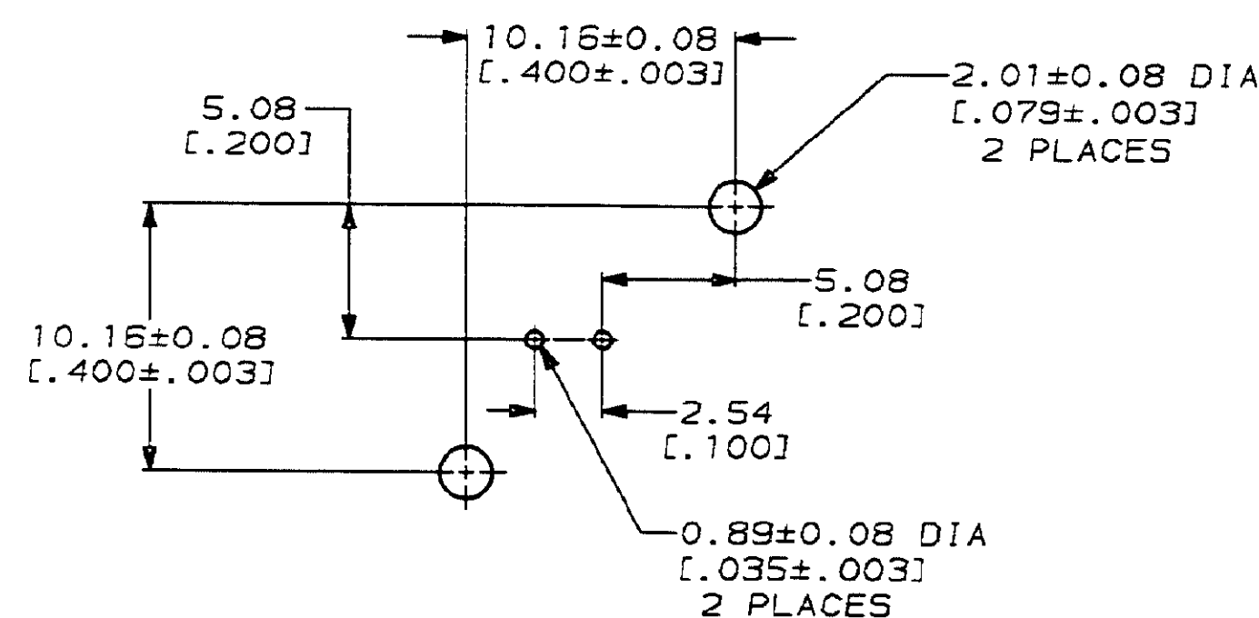
PCB CONFIGURATION
