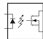
1-Form-A Unidirectional
