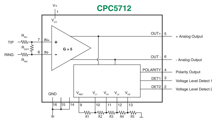
Resistors set the Voltage Level Detect Thresholds
