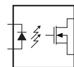
1-Form-B Unidirectional
