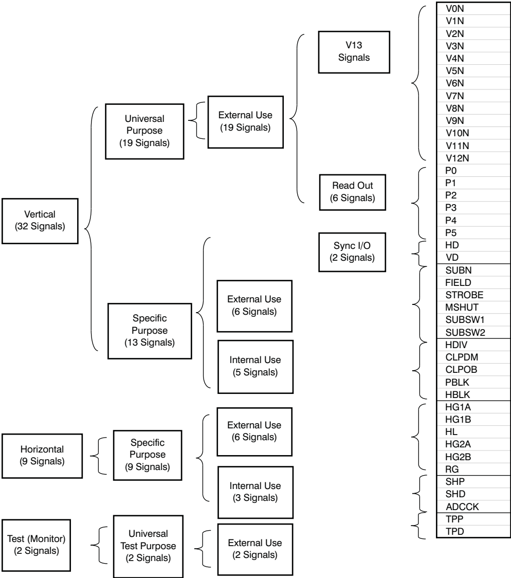
Figure 28. Signal Overview
