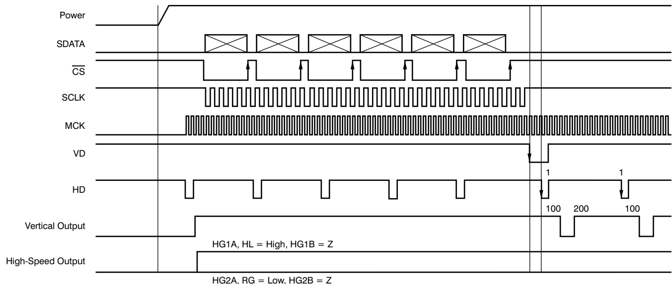
Figure 17. Power-Up Sequence
