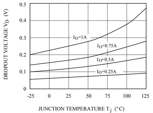
Fig.8 T_j - V_D
