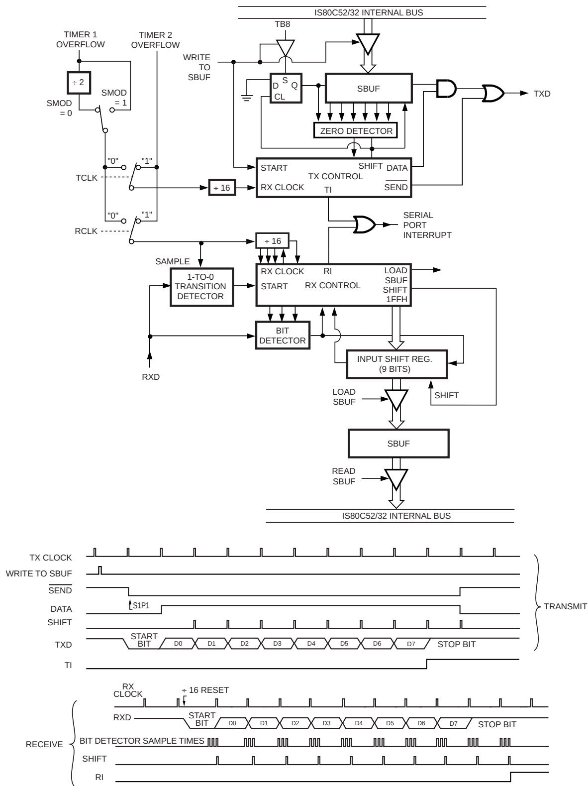
Figure 16. Serial Port Mode 1
