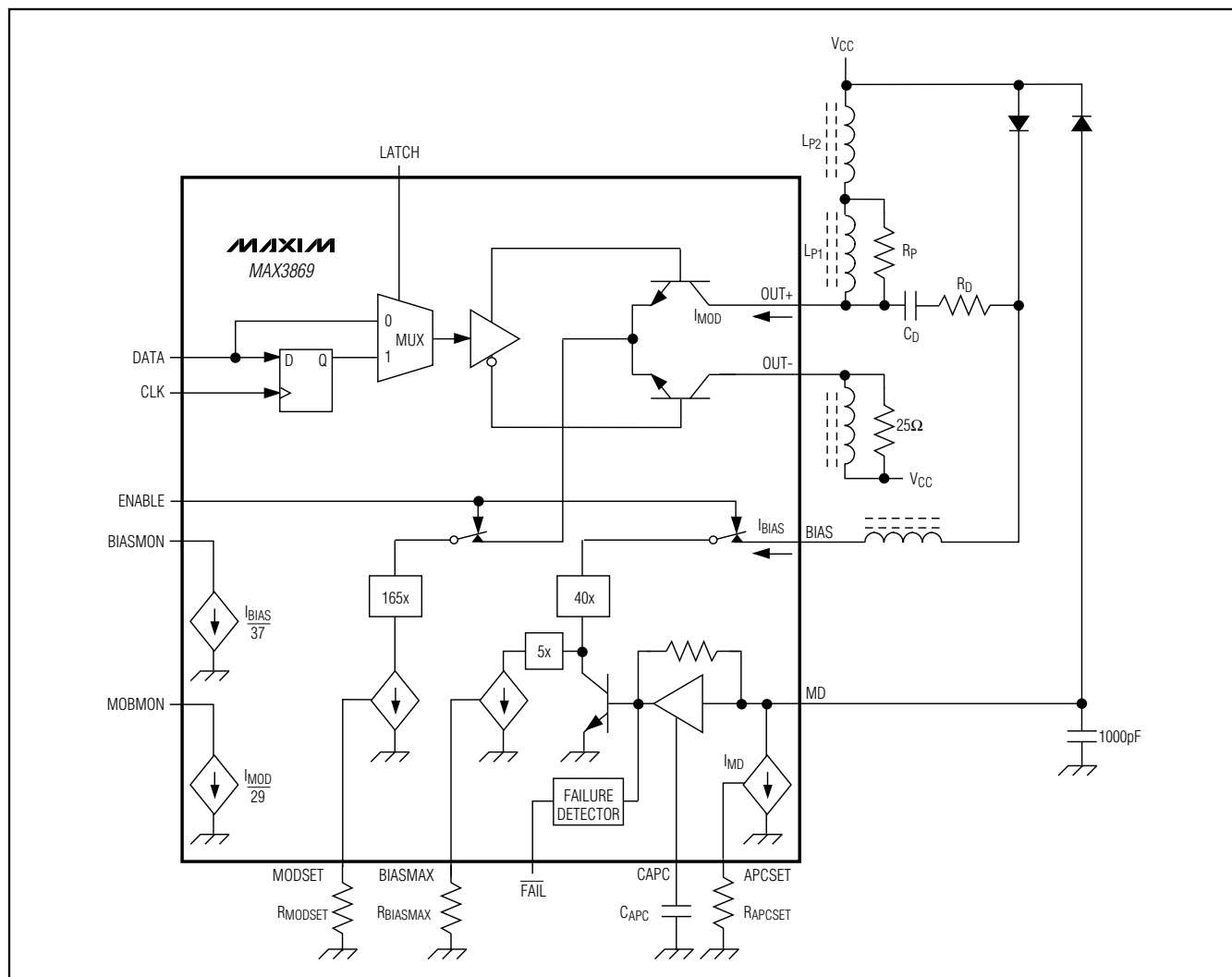
Figure 4. Functional Diagram
