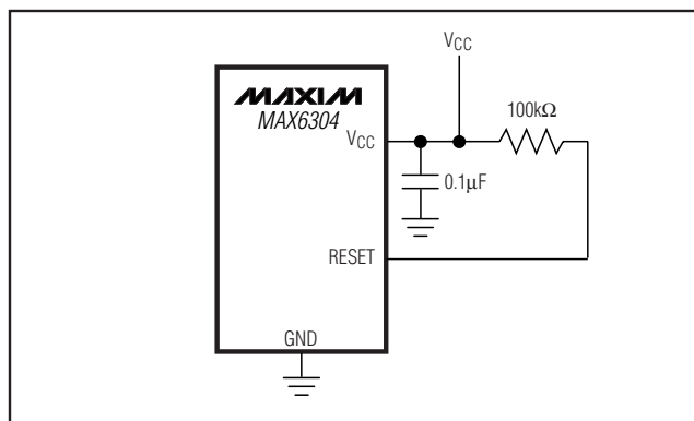
Figure 10. Ensuring \overline{\text{RESET}} Valid to V_{CC} = 0V
