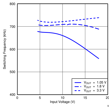
Figure 8-7. Switching Frequency vs Input Voltage ( I_O = 1\text{ A} )
