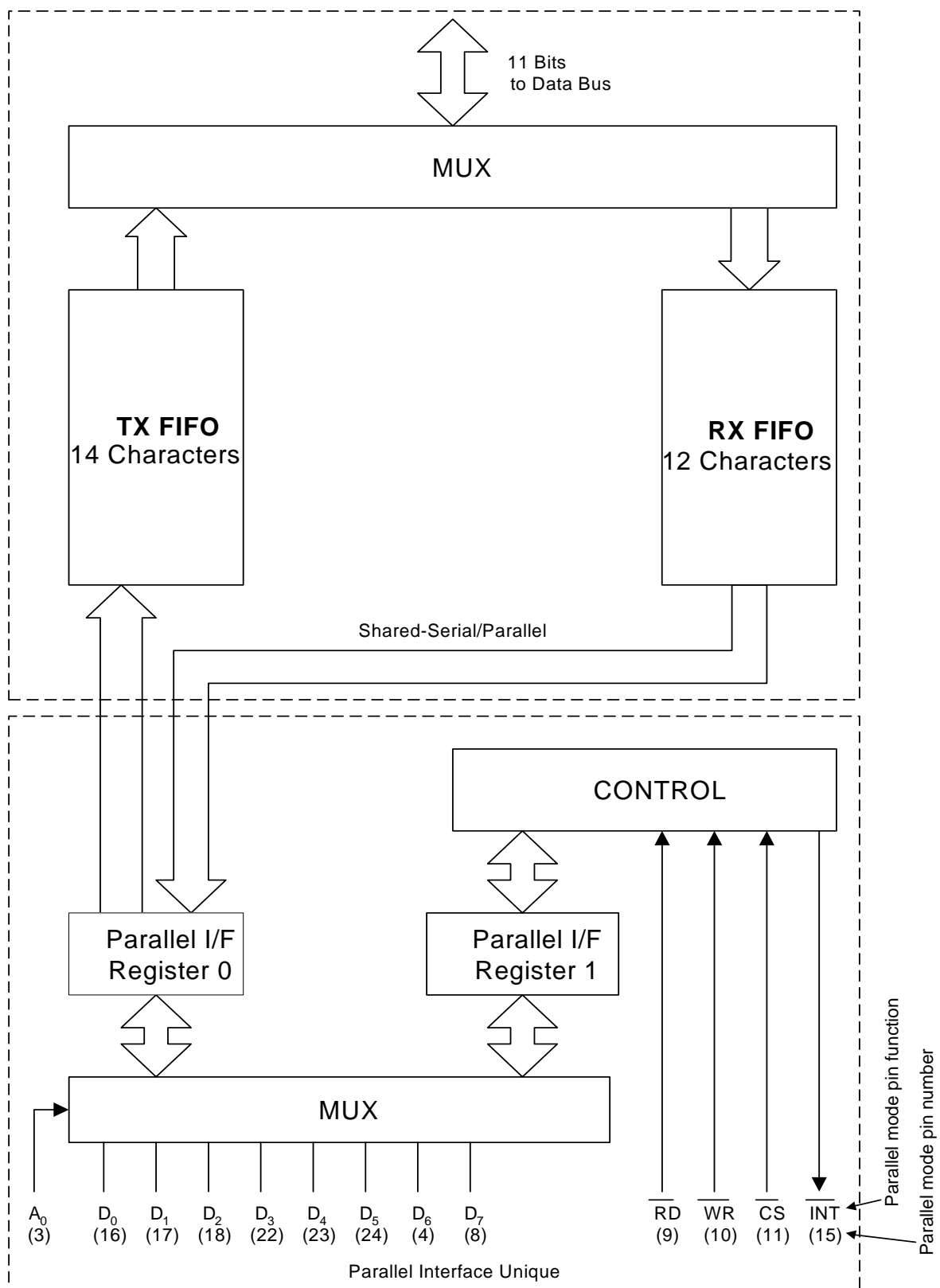
Figure 6. Parallel Interface
