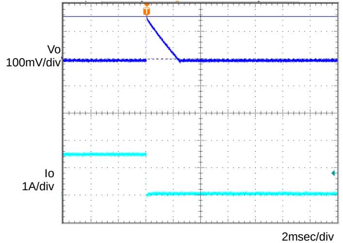
Figure 8. Transient Response (1.0→0A) C_o = 1\mu\text{F} , T_a = 105^\circ\text{C}
