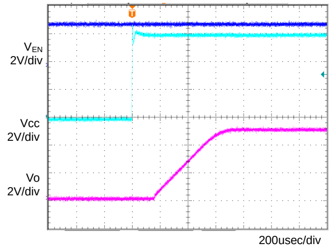
Figure 10. Input sequence 1 C_o = 1\mu\text{F} , T_a = 25^\circ\text{C}
