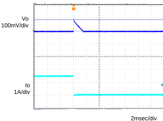
Figure 6. Transient Response (1.0→0A) C_o=1\mu F , T_a=-40^\circ C
