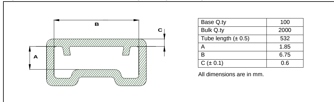
Figure 40. PowerSSO-16 tube shipment (no suffix)
