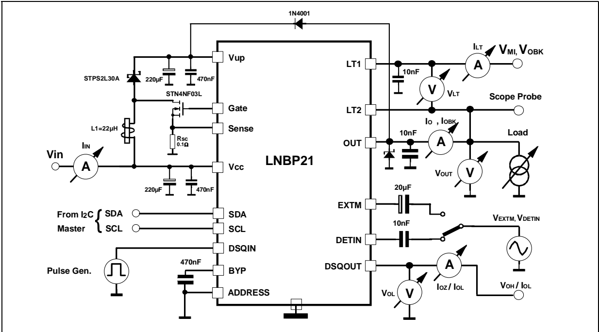
Figure 7: Test Circuit
