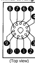
Terminal arrangement
