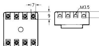
Terminal arrangement
