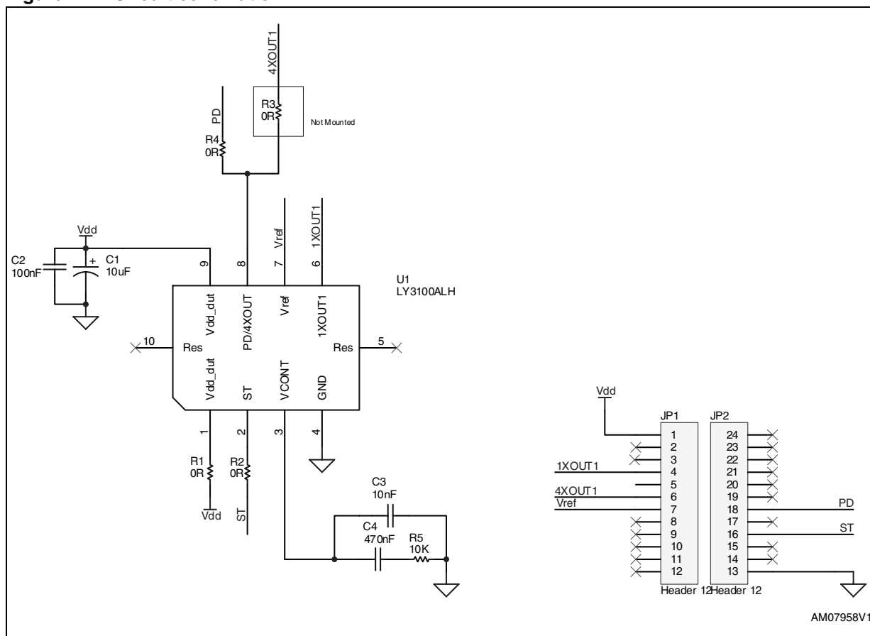
Figure 1. Circuit schematic
