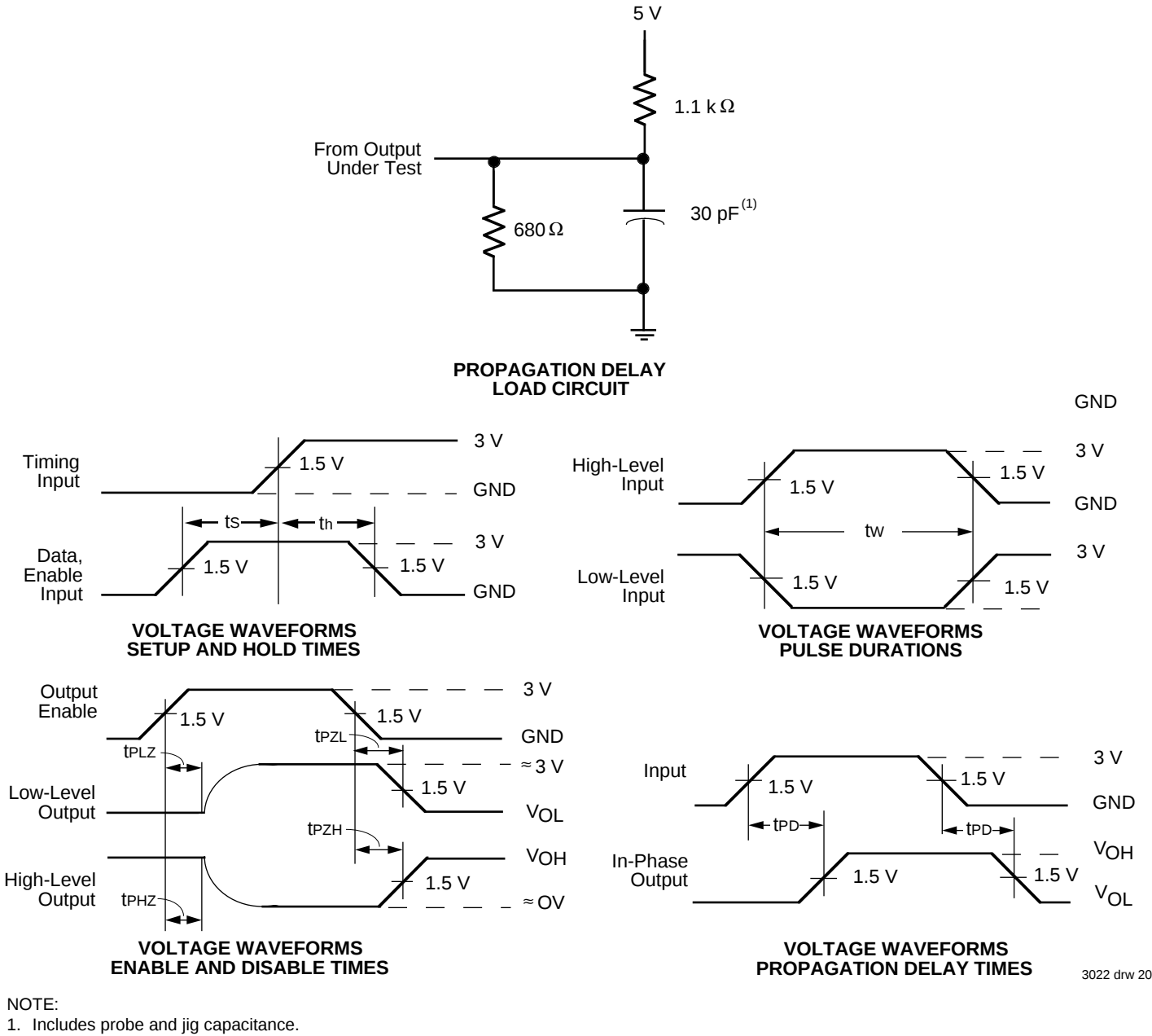
Figure 18. Load Circuit and Voltage Waveforms.
