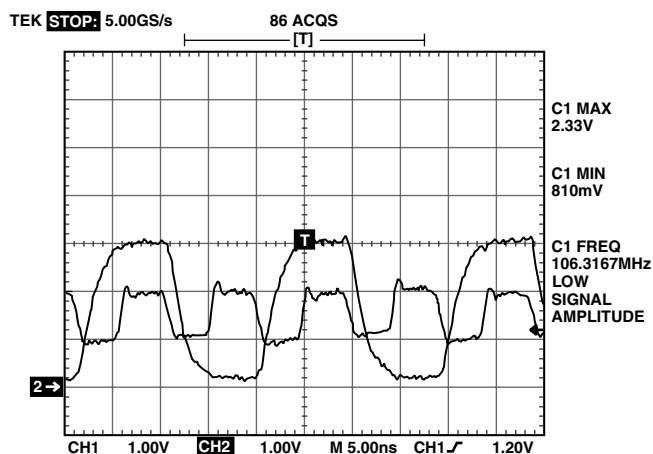
Figure 15. Encode+ Clock and Latch Clock
