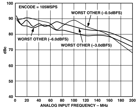
TPC 6. Worst-Case Spur (Other than Second and Third) vs. f_{IN} : f_s = 105 \text{ MSPS}
