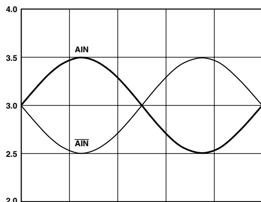
Figure 7. Full-Scale Analog Input Range
