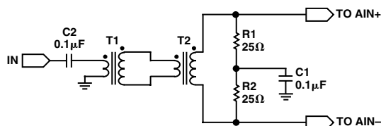
Figure 13. Improving Second Harmonic Distortion Performance
