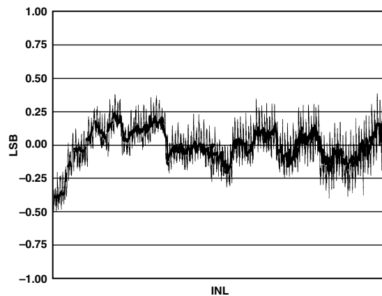
TPC 15. Integral Nonlinearity: f_s = 105 \text{ MSPS}
