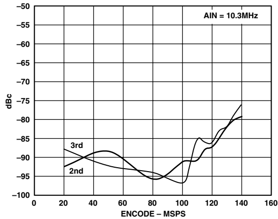
TPC 2. Harmonics vs. f_s : f_{IN} = 10.3 \text{ MHz}
