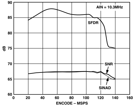
TPC 1. SNR/SINAD/SFDR vs. f_s : f_{IN} = 10.3 \text{ MHz}
