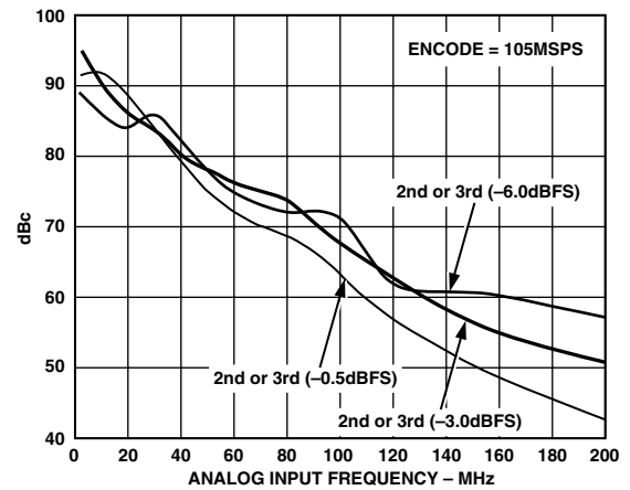
TPC 5. Harmonics vs. f_{IN} : f_s = 105 \text{ MSPS}
