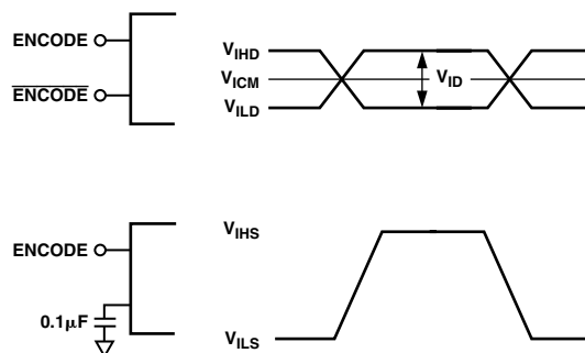
Figure 9. Differential and Single-Ended Input Levels
