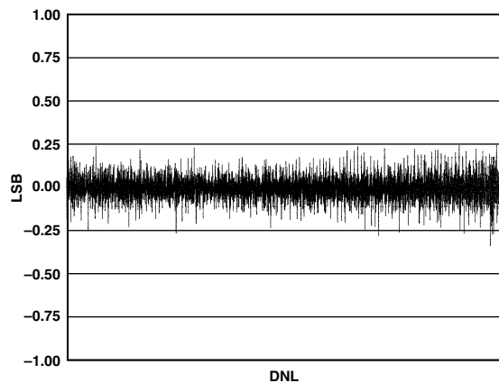
TPC 14. Differential Nonlinearity: f_s = 105 \text{ MSPS}
