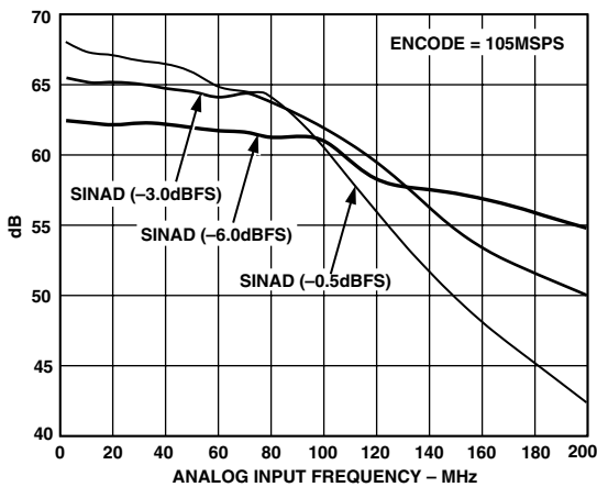
TPC 3. SINAD vs. f_{IN} : f_s = 105 \text{ MSPS}
