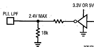
Figure 9. Directly Driving PLL LPF Pin
