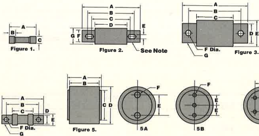
Rectifier Fuses—Dimensional, Carton Quality and Weight Data
