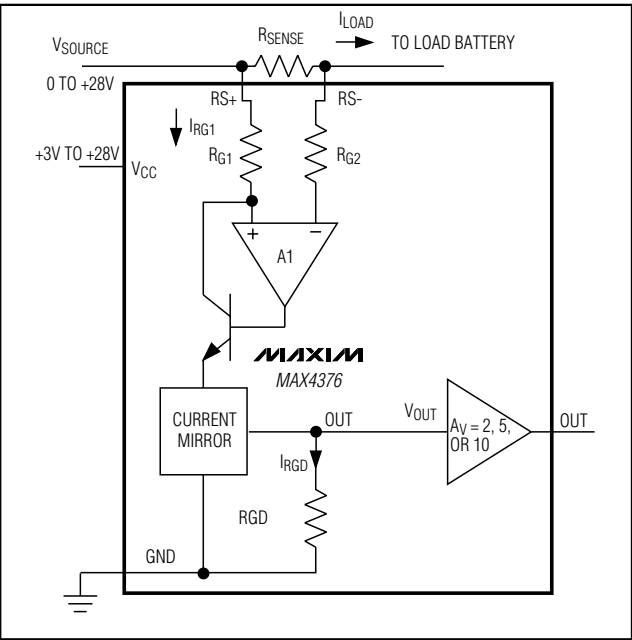
Figure 1. Functional Diagram
