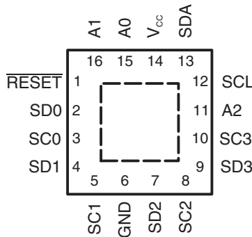
RGV PACKAGE (TOP VIEW)
