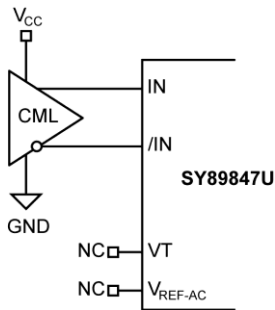
Figure 4c. CML Interface (DC-Coupled)
