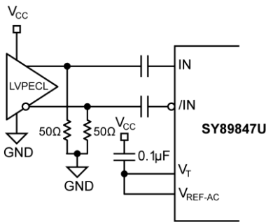
Figure 4b. LVPECL Interface (AC-Coupled)
