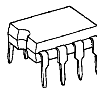
DIP8-P-300-2.54C
