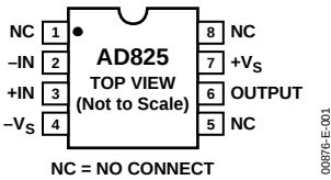
Figure 4. 8-Lead SOIC
