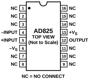
Figure 5. 16-Lead SOIC
