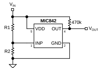
Figure 2. Example Circuit
