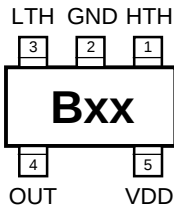
MIC841 SC-70-5 (C5)
