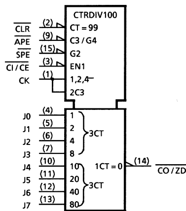
TC74HC40102A
