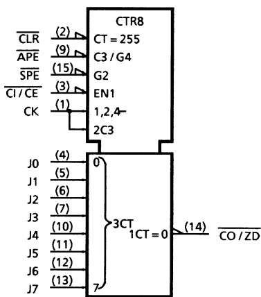
TC74HC40103A
