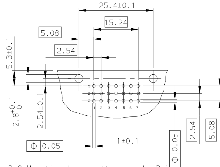
P.C.Mounting hole pattern scale 2:1
