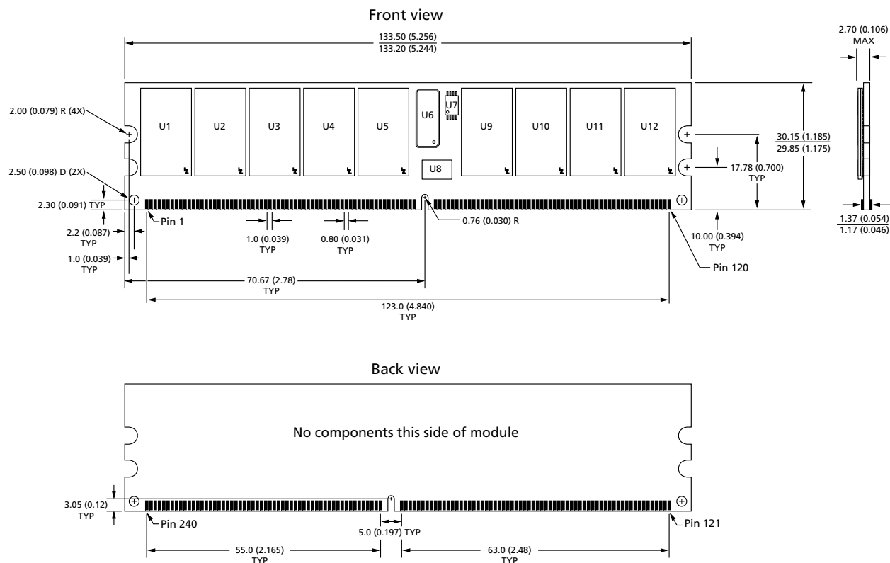
Figure 4: 240-Pin DDR2 RDIMM
