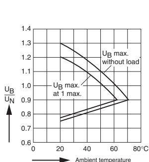
Relay operation voltage vs. ambient temperature
