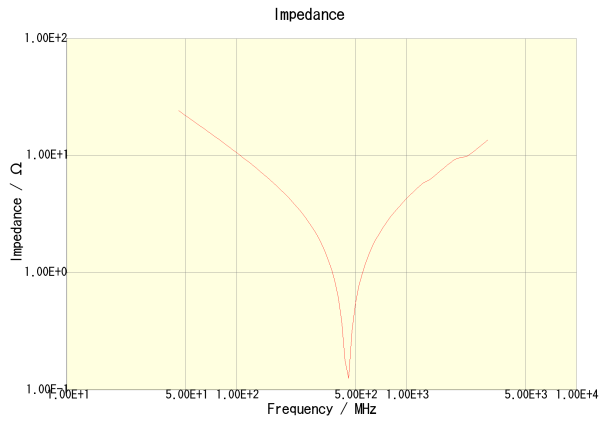
C1608C0G2E151J080AA
