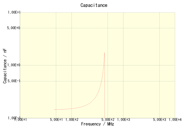
C1608C0G2E151J080AA
