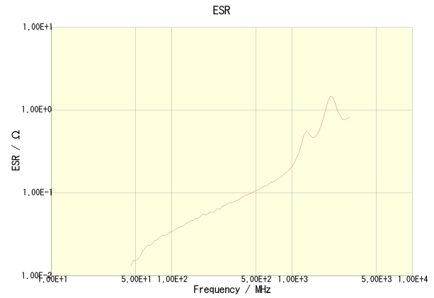
C1608C0G2E151J080AA
