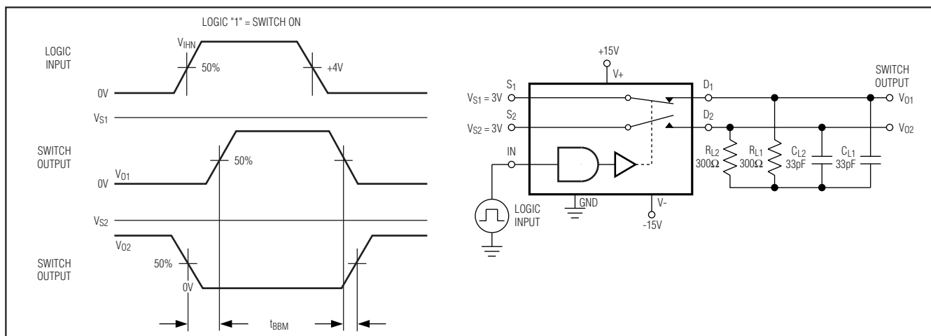
Figure 2. Break-Before-Make Time Test Circuit SPDT (DG301(A), DG303(A))
