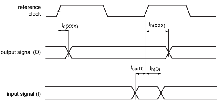
Fig 26. UART timing
