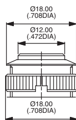
Flat actuator AV6P30C9
