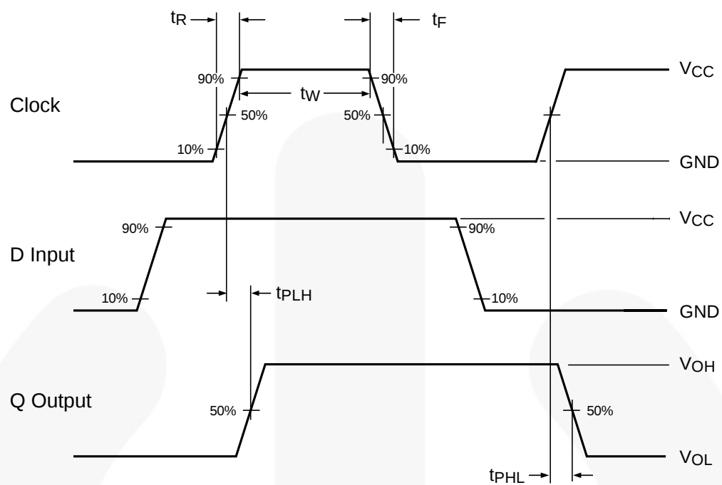
Figure 3. AC Waveform
