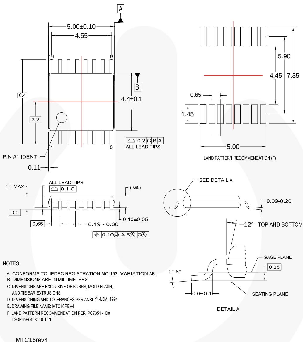
Figure 6. 16-Lead Thin Shrink Small Outline Package (TSSOP)
