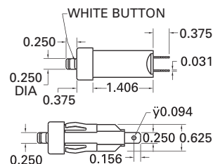
With Front Mount Clip Installed
