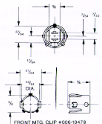
FRONT MTG. CLIP #006-10478
