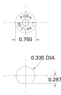
PANEL MTG. HOLE FOR PANEL THICKNESS 1/32 THRU 1/8
