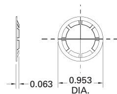
#006-10417 Retaining Ring
