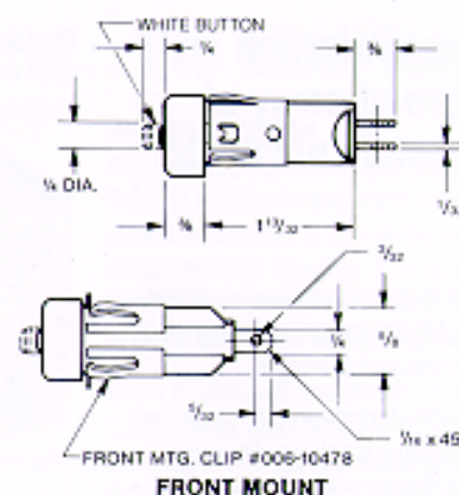
FRONT MOUNT
