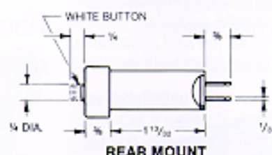
REAR MOUNT
