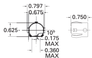
#006-10478 Front Mount Clip
