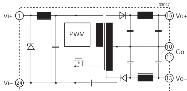
Fig. 4 Block diagram for dual-output models with alternative pinout (option K).
