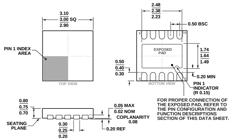
Figure 48. 10-Lead Lead Frame Chip Scale Package [LFCSP_WD] 3 mm × 3 mm Body, Very Very Thin, Dual Lead (CP-10-9) Dimensions shown in millimeters
