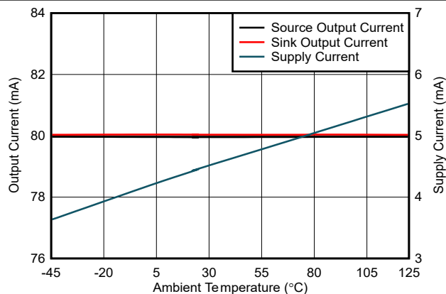
Figure 6-12. Supply and Output Current vs Temperature
