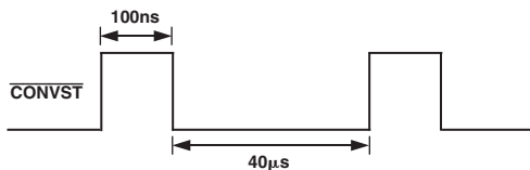
Figure 17. \overline{\text{CONVST}} When Temperature Channel Selected
