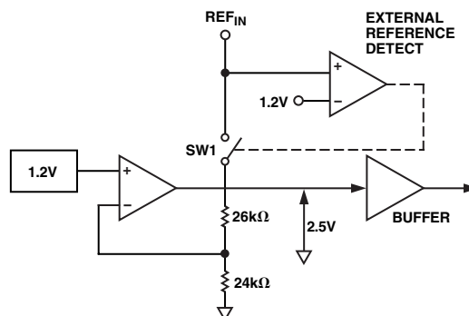
Figure 4. On-Chip Reference
