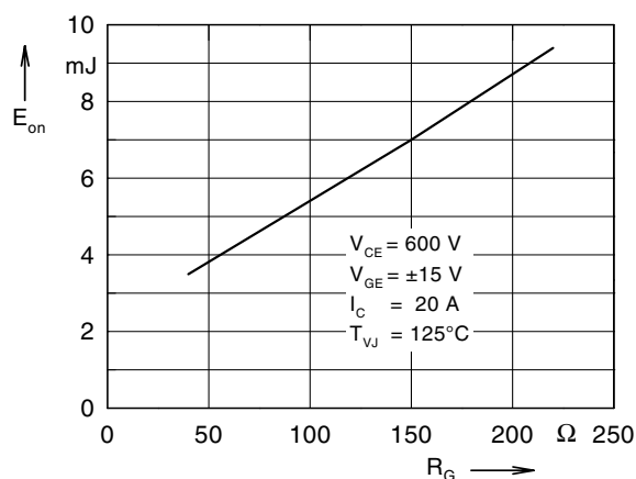
Fig. 9 Typ. turn on energy vs gate resistor
