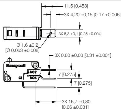
FIGURE 8. V15 SERIES N-STYLE RAST-7 250# CONNECTOR
