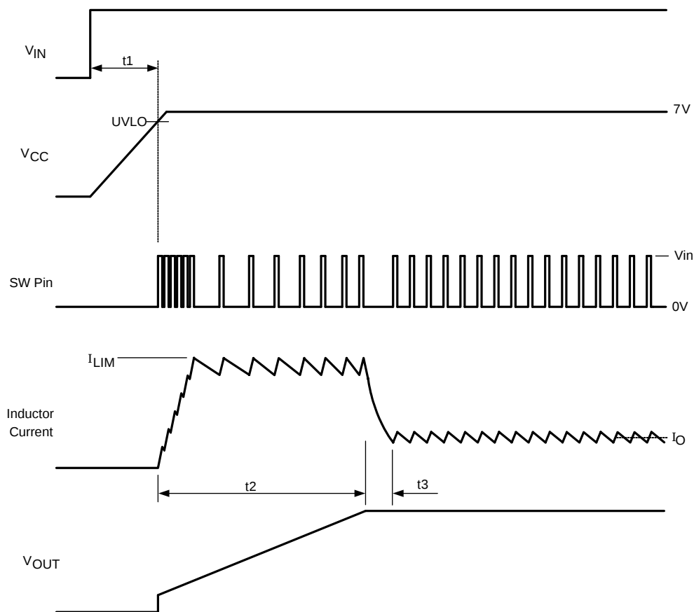
Figure 8. Start-Up Sequence
